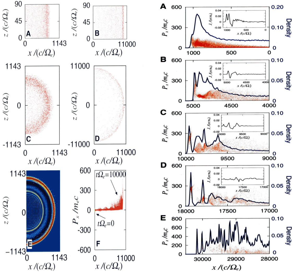
Fig. 3. (left) 2.5D PIC simulations of slab and cylindrical e^+e^- plasma acceleration, with initial plasma temperature kT=5 MeV, \Omega_e/\omega_{pe}=10 ( \Omega_e = eB_o/m_e , \omega_{pe} = (n_e^2/\epsilon_o m_e)^{1/2} ), initial slab width L_o = 120c/\Omega_e and uniform internal \mathbf{B}=(0, B_o, 0) . We show the x \geq 0 snapshots of particle distribution (a-d), axial magnetic field (color scale runs from \mathbf{B}_y = +0.2B_o (red) to -0.1B_o (blue)) and current density (white arrows) for the cylindrical case (e), and phase plot for the slab case (f). \Omega_e t = 800 for all left panels and \Omega_e t = 10^4 for all right panels. The green dot in the phase plot denotes the initial phase volume (from Liang & Nishimura 2004).
