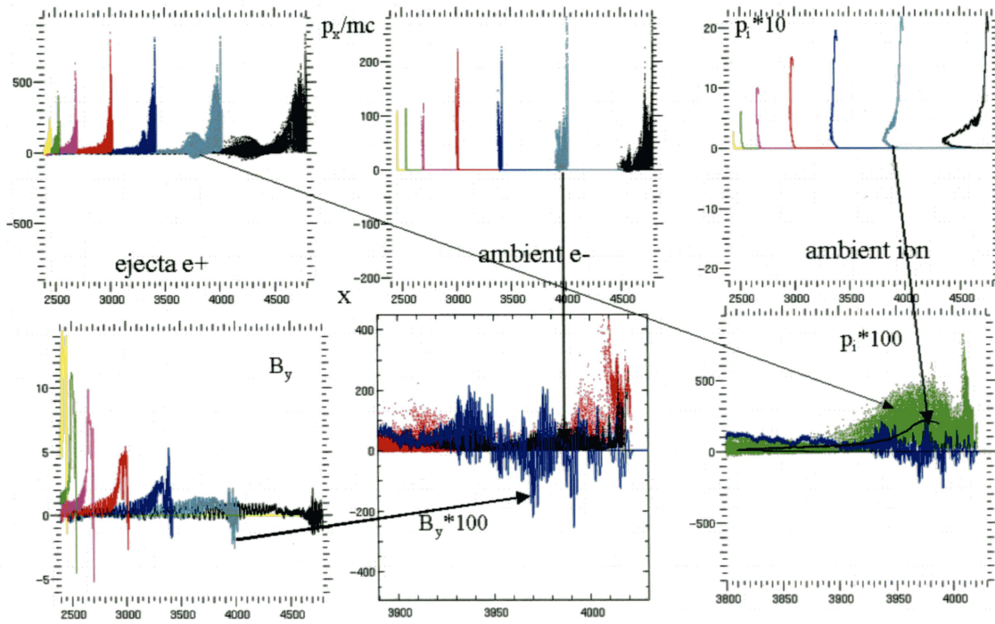
Fig. 13. Time-lapse phase plots and B-field profiles for a slab e^+e^- 2.5D DRPA running into (0.001 \times ejecta density) cold e^- ion ambient plasma. P_i is in units of m_e c . The acceleration of ejecta plasma stalls after it has swept up roughly equal mass of ambient plasma but the acceleration of ambient ions continues due to the pull by charge separation Ex. EM field decays by acceleration of swept-up plasma and mode conversion. Lower right panels show the blow-up details of the transition region (from Liang 2005).
