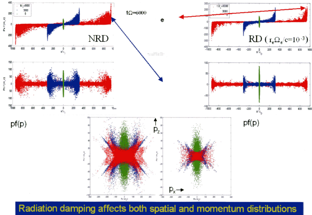
Fig. 9. Phase plots and density profiles of a no-RD run compared to an RD run (same input parameters as in Fig. 3a (from Liang 2005)).
