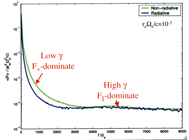
Fig. 10. Comparison of average radiation output per electron computed from the runs of Fig. 9 (from Noguchi et al. 2005).
