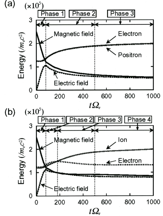
Fig. 2. Time evolution of the magnetic field, electric field, and particle energies for (a) the electron-positron DRPA expansion; (b) the electron-ion expansion (from Liang et al. 2003).
