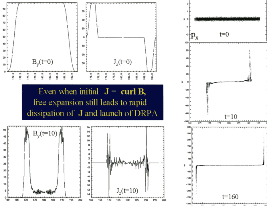
Fig. 7. Evolution of B_y, J_z and phase plot of e^+e^- slab expansion as in Fig. 3a, but with initial \mathbf{J}=\text{curl } \mathbf{B} . The late time phase plot is almost identical to that of DRPA (here t=t\Omega_e/30 ) (Liang 2005).
