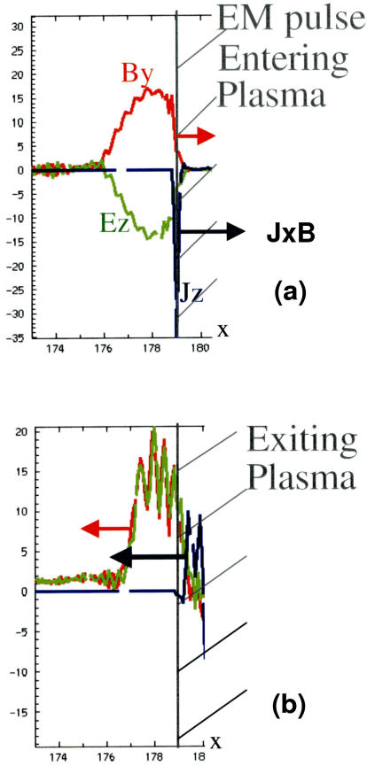
Fig. 1. Schematics showing the \mathbf{J} \times \mathbf{B} forces (black arrow) when an EM pulse tries to enter a plasma (a) and when it tries to leave a plasma (b). DRPA is based on the second scenario.
