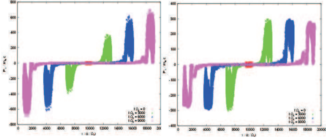
Fig. 12. Evolution of \Omega_e/\omega_{pe}=100 DRPA phase plots including Comptonization of external blackbody soft photons. Left panel is for low photon density and right panel is for high photon density, showing the rapid decline of the maximum Lorentz factors (Sugiyama unpublished).
