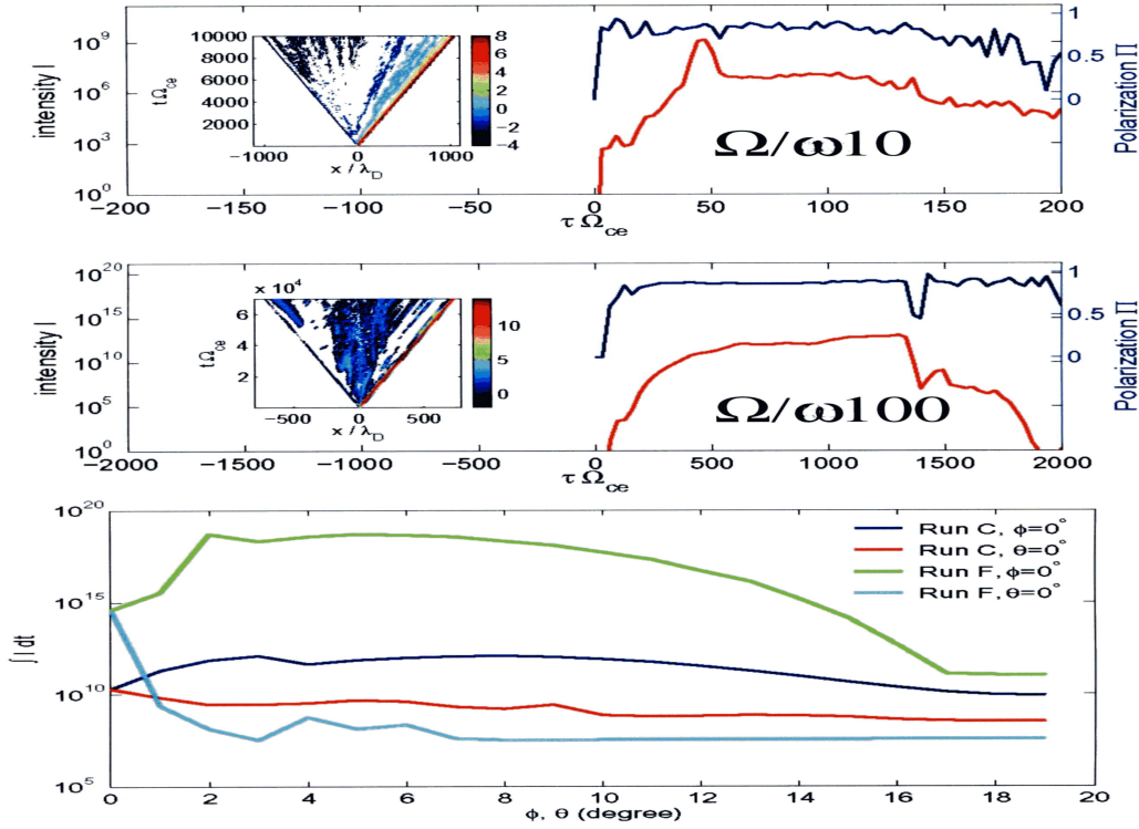
Fig. 11. Detected radiation intensities and polarization as functions of detector time for \Omega_e/\omega_{pe}=10 and \Omega_e/\omega_{pe}=100 runs including RD using ray-tracing (upper panels). Bottom panel is detected angular fluence plotted against view angle ( \theta in x-z plane and \phi in x-y plane) (Noguchi et al. 2005).
