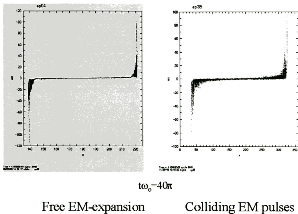
Fig. 8. Late-time phase plot of e^+e^- slab accelerated by colliding vacuum EM pulses (right) is almost identical to that of DRPA (left) (Liang 2005).
