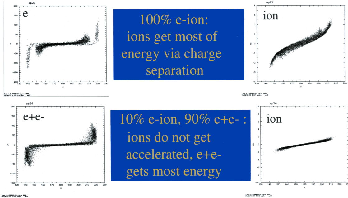
Fig. 14. Phase plots of the electrons and ions for a mixture of 10% e-ion and 90% e + e - plasma compared to pure e-ion plasma (from Liang 2005).
