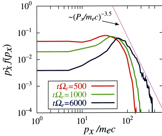
Fig. 5. Evolution of the x-momentum distribution for all surface particles in the slab DRPA of Fig3a, showing the peak Lorentz factor \gamma_m (=p_{xmax}/m_e c) increasing with time and a power law of slope \sim -3.5 at \Omega_e t = 6000 (from Liang & Nishimura 2004).
