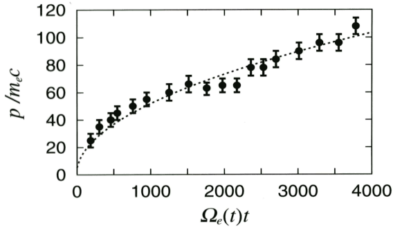
Fig. 6. The peak Lorentz factor \gamma_m versus time for the slab pulse, compared with Eq.(1). The best-fit curve (dotted) gives f=1.33 and C_o=27.9 . Note that \Omega_e(t) \cdot t = 3800 is equivalent to \Omega_e \cdot t = 18000 due to B decay. This result shows that for t > L_o/c , \gamma_m scales as the square-root of the number of gyroperiods (from Liang and Nishimura 2004).
