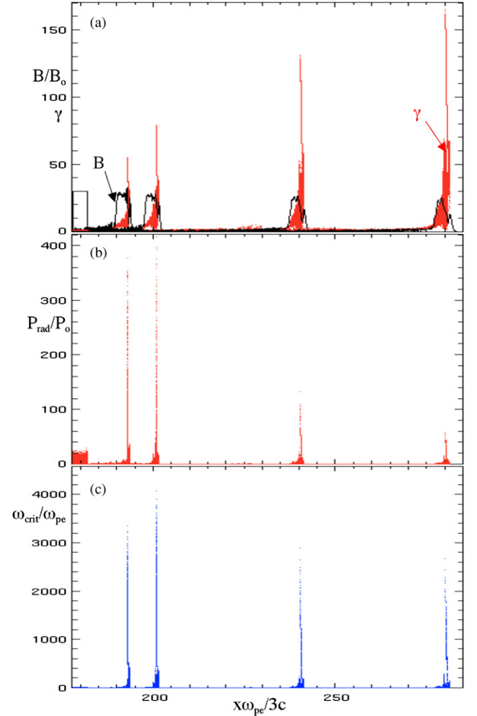
Figure 4. Snapshots at different times of the spatial profiles of a pair-loaded EM pulse propagating from left to right show the CPFA evolution. The e^+e^- plasma slab has initial temperature kT_o = 0.005 m, pulse width L_o = 12 c/\omega_{pe} , \Omega_e/\omega_{pe} = 10 , and was initially located at x\omega_{pe}/3c = 180 . The five snapshots (left to right) are taken at t\omega_{pe}/3 = 0, 12, 20, 60, 100 . We show the scatter plot for 1% of all superparticles. (a) Time evolution of the magnetic field B_y and electron Lorentz factors \gamma spatial distributions shows monotonic increase in \gamma and conversion of magnetic energy into particle energy via current dissipation. (b) Evolution of P_{\text{rad}} spatial distribution shows that radiation loss for the highest energy electrons peaks at \sim 5 light crossing times, followed by monotonic decay when the increase in \gamma is countered by the decrease in B and \sin\alpha . (c) Evolution of the critical frequency \omega_{\text{cr}} spatial distribution shows a similar trend. \omega_{\text{cr}} is expressed in units of \omega_{pe} = 0.1\Omega_e .
